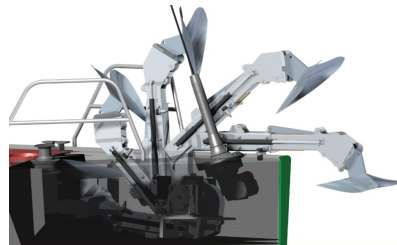
ACTUATED ANCHOR SYSTEM
